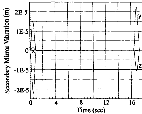
e) Secondary mirror vibration
