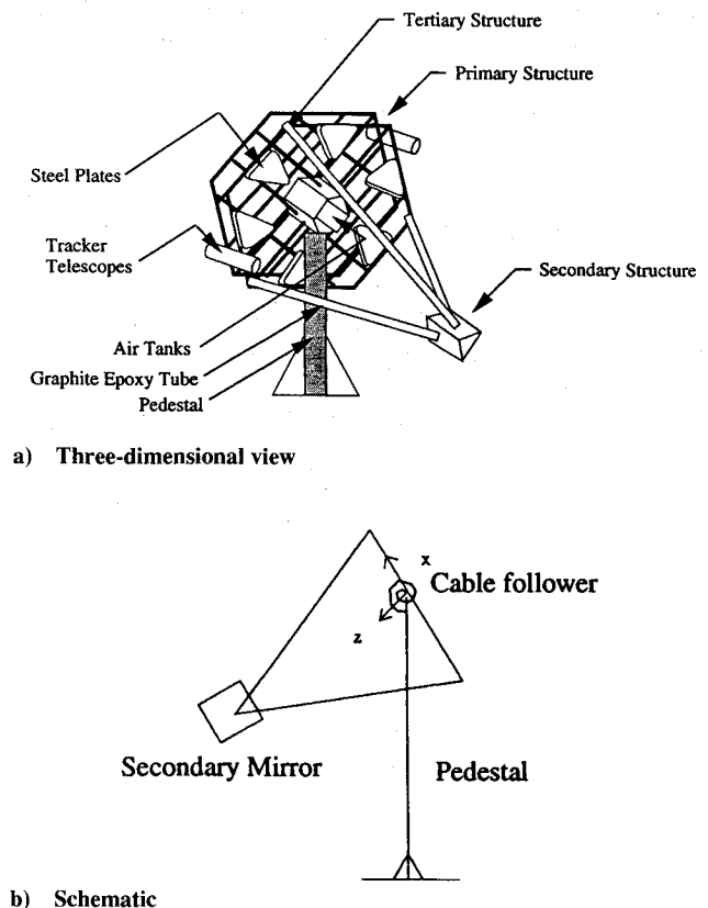
Fig. 1 ASTREX test article.
